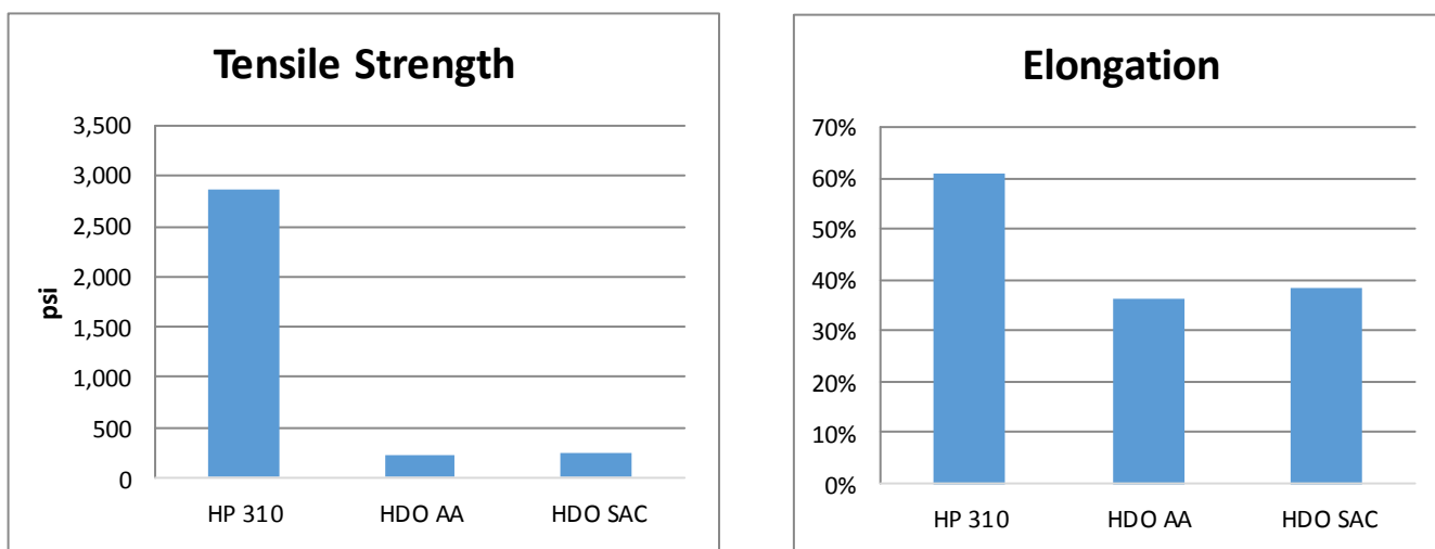
Figure 1: Tensile strength and elongation of Myrinol™ HP 310 compared to traditional hexanediol adipate (HDO AA) and hexanediol succinate (HDO SAC).
